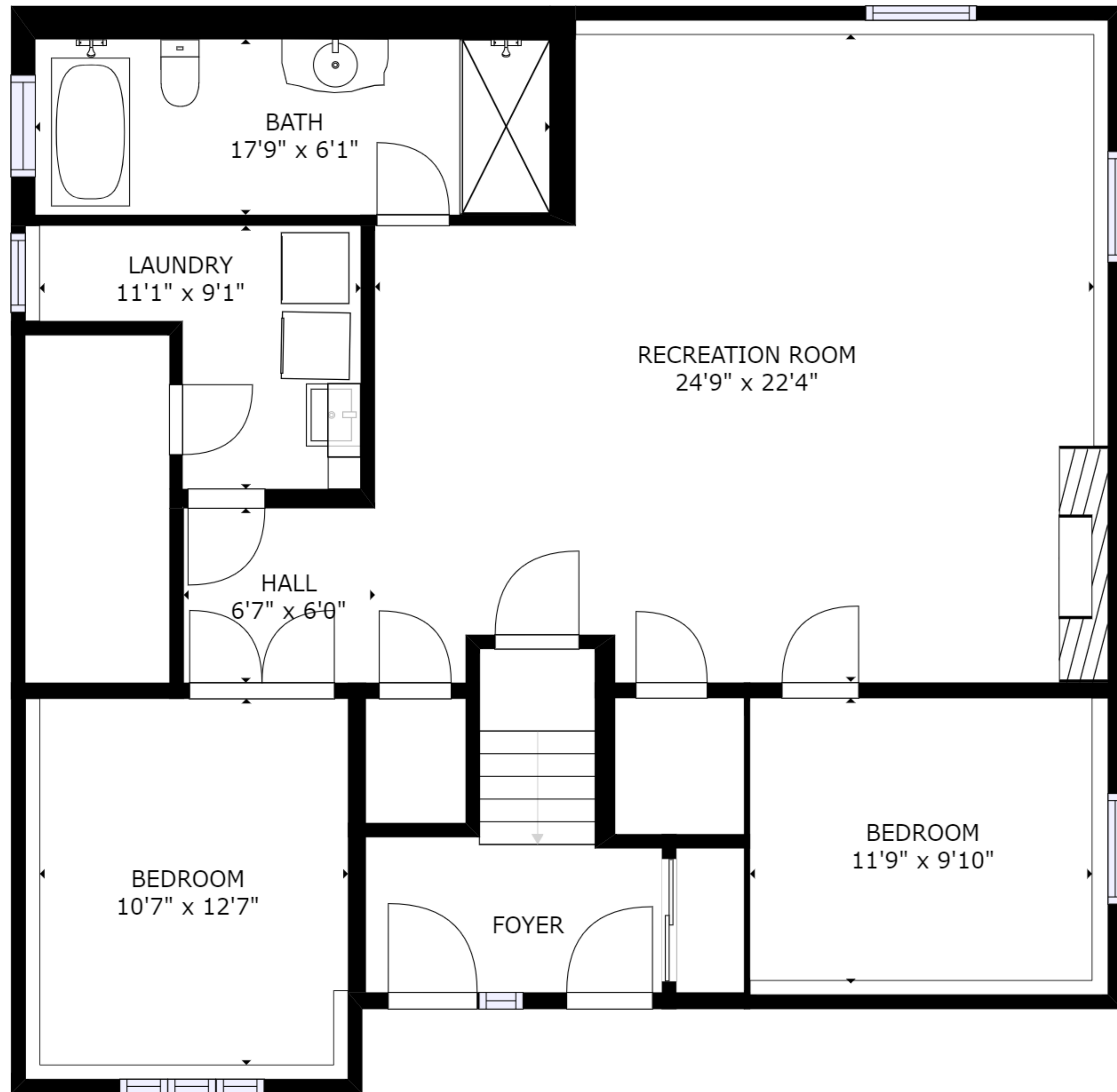
FLOOR 1
