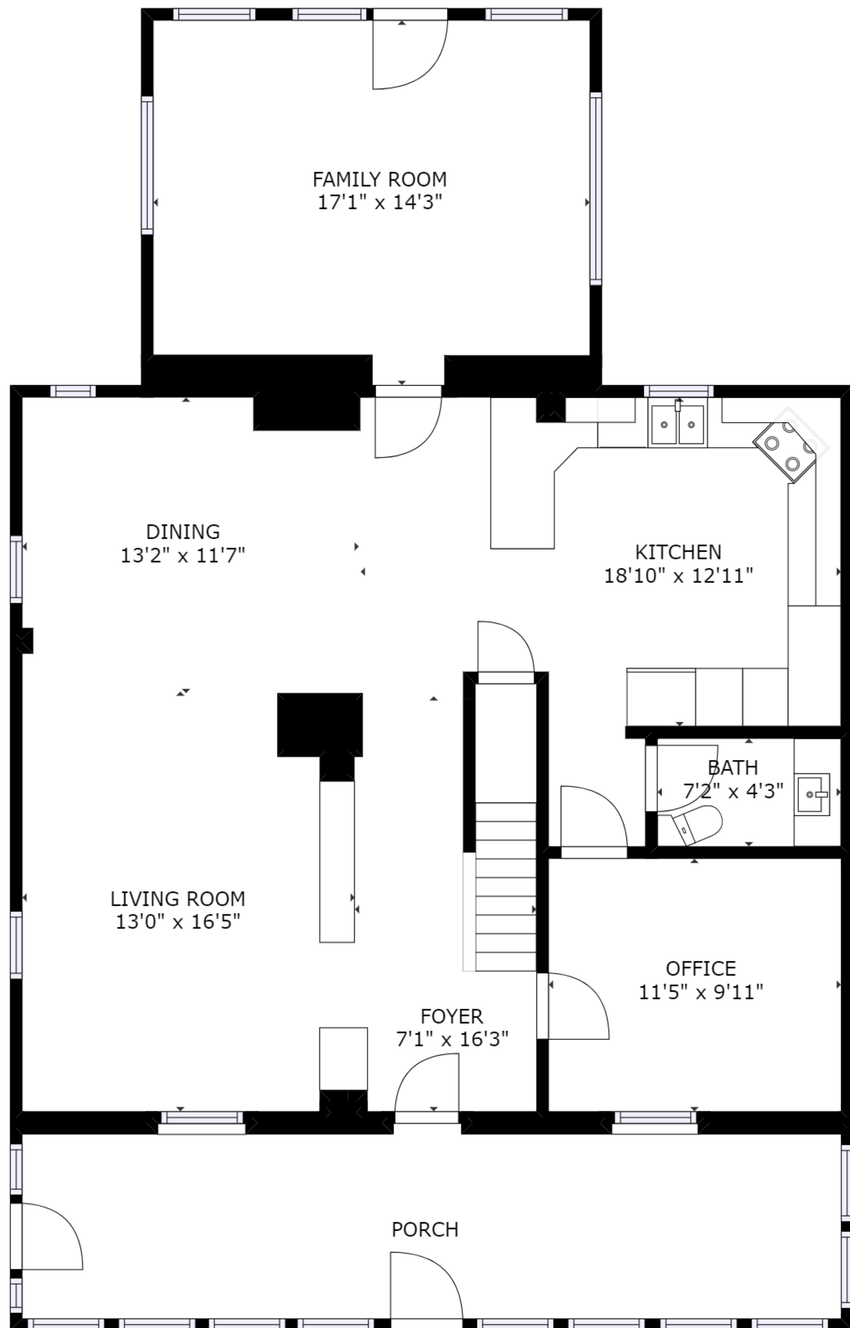
FLOOR 1
