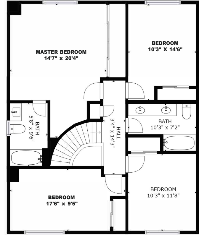
UPSTAIRS
