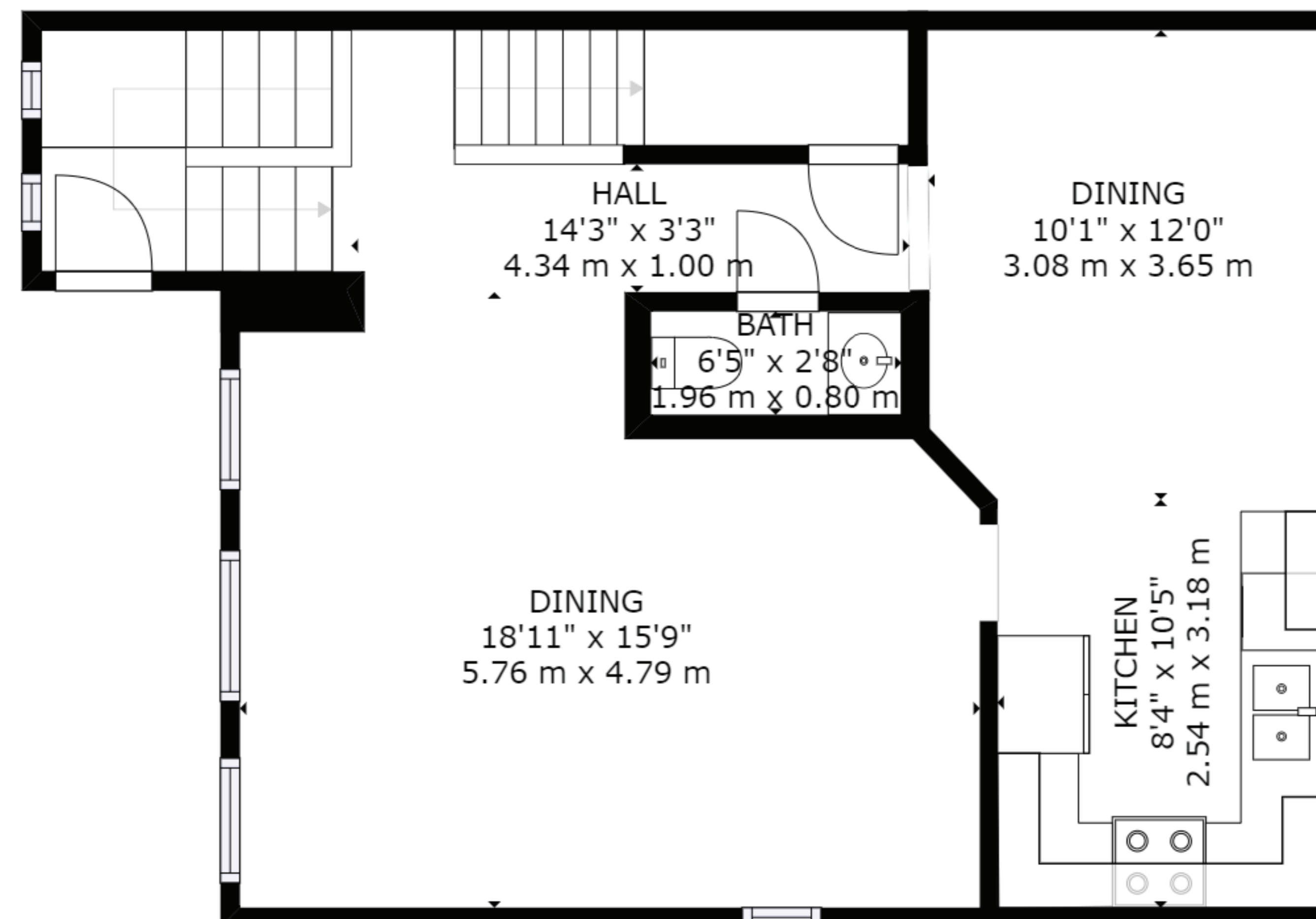
MAIN FLOOR
