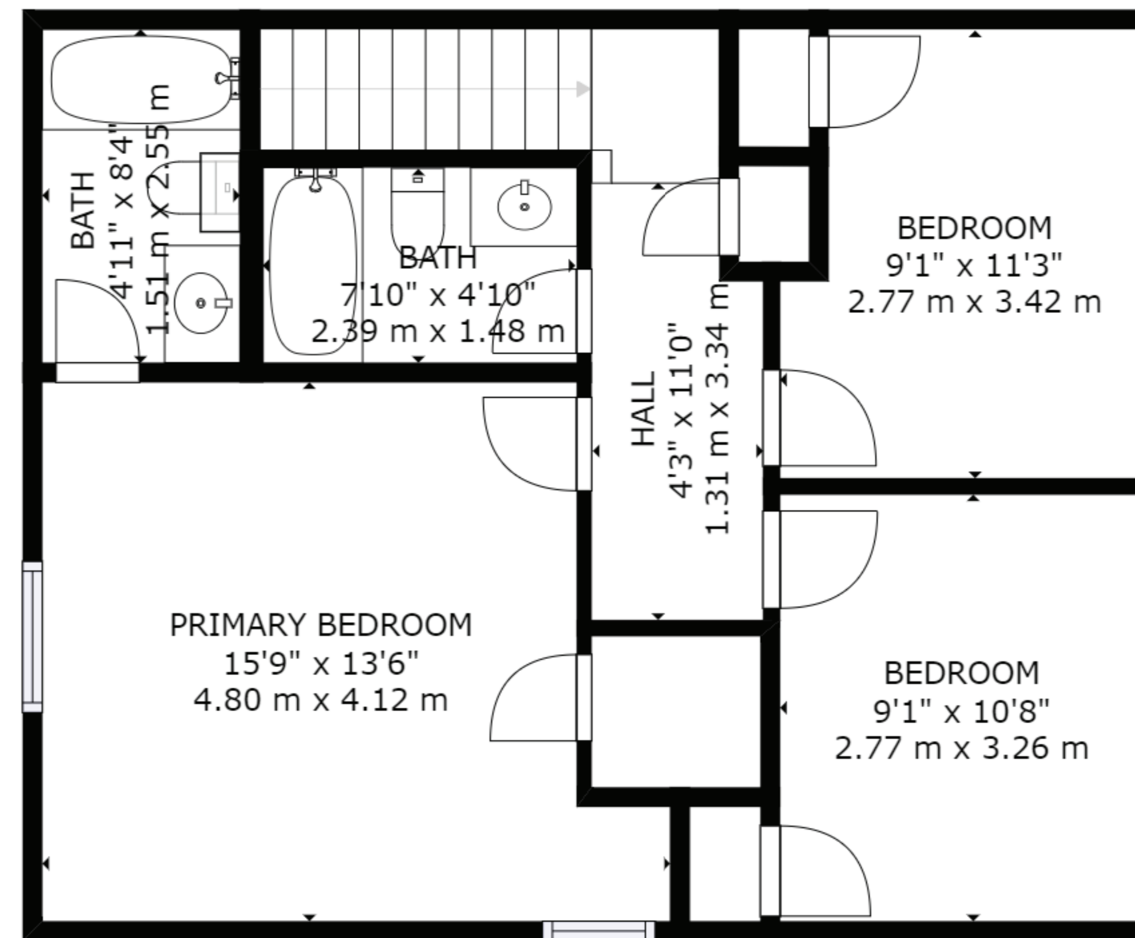
SECOND FLOOR
