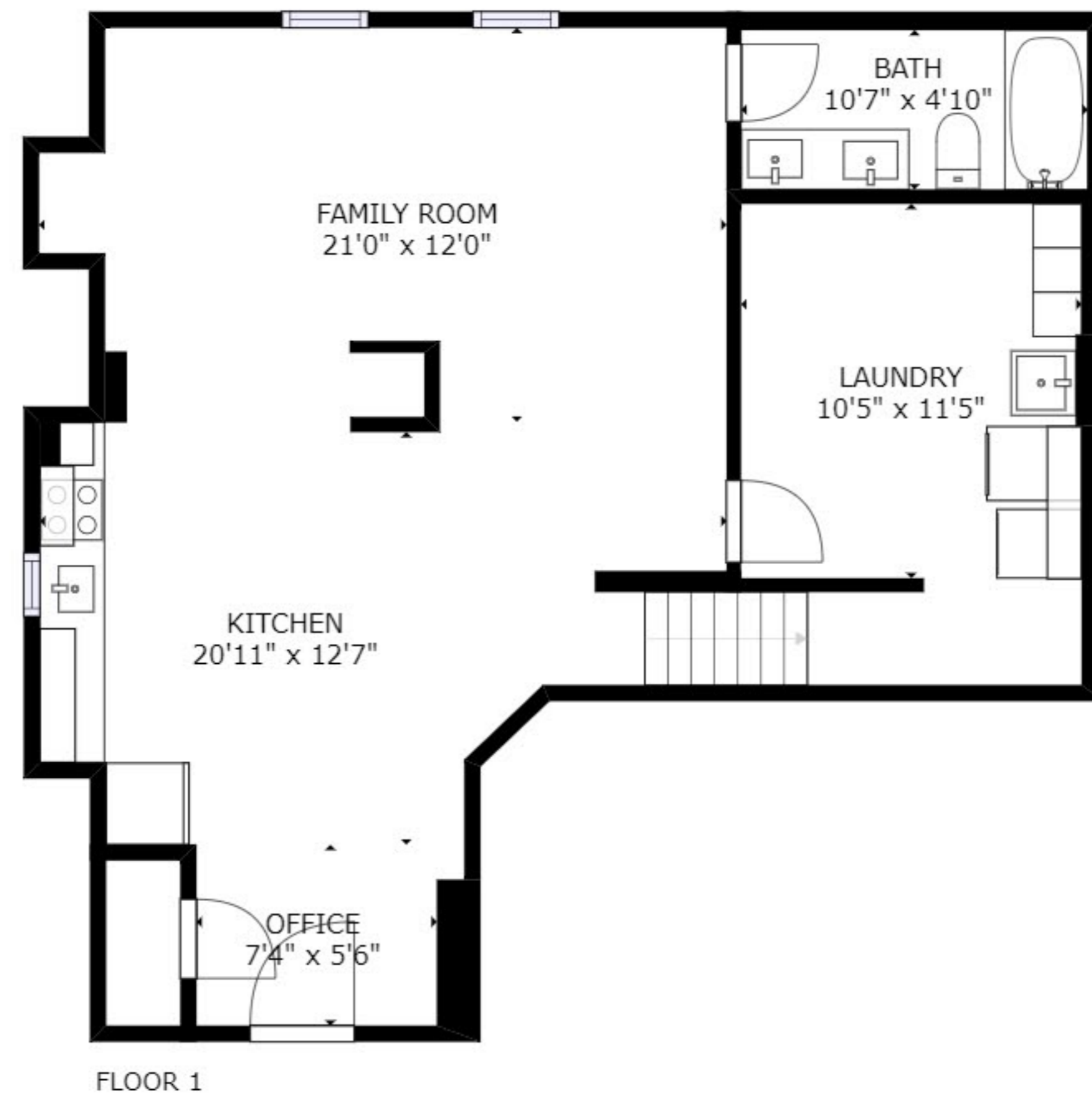
FLOOR 1
