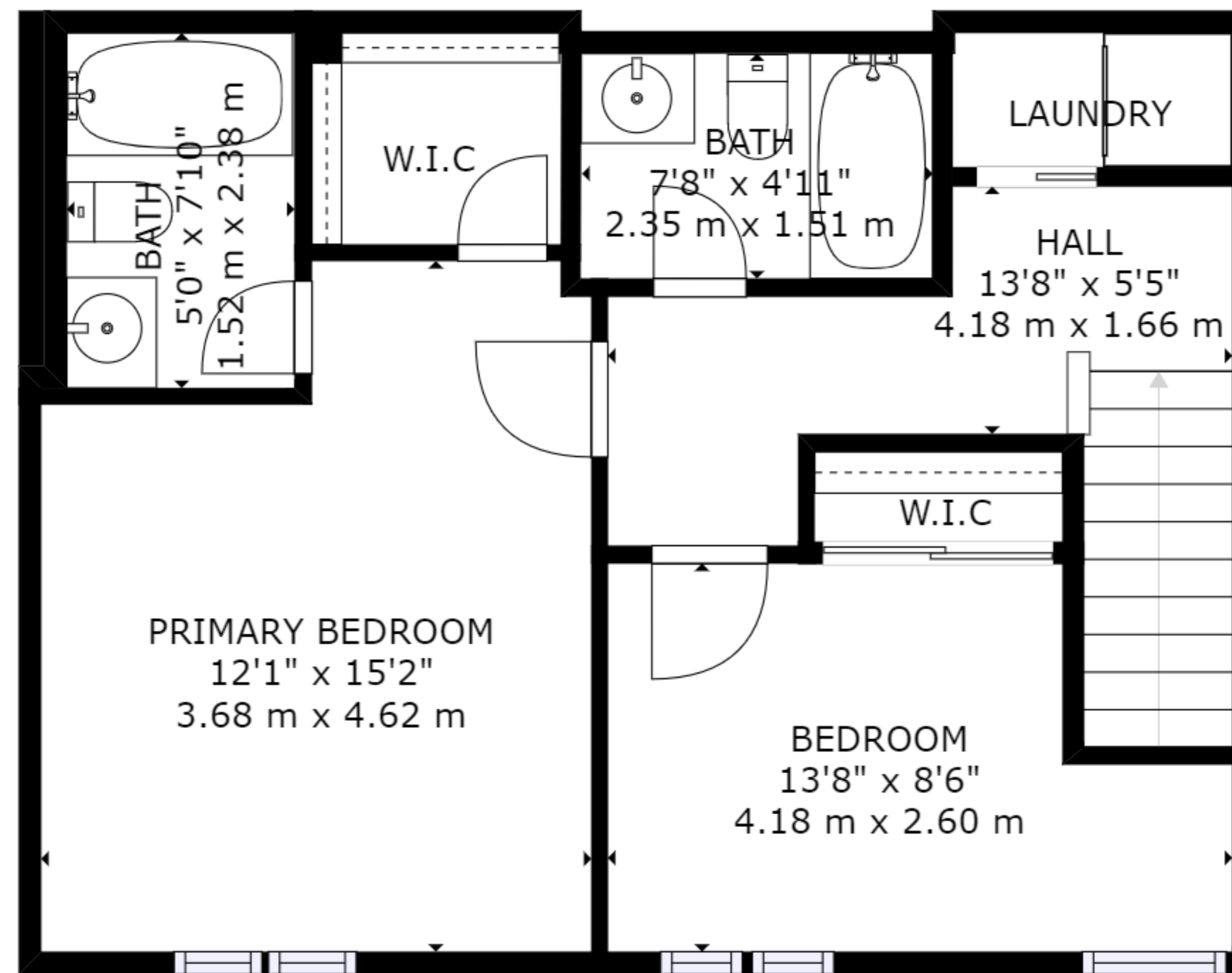
FLOOR 3
