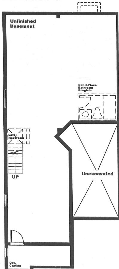
Basement Elevation C
