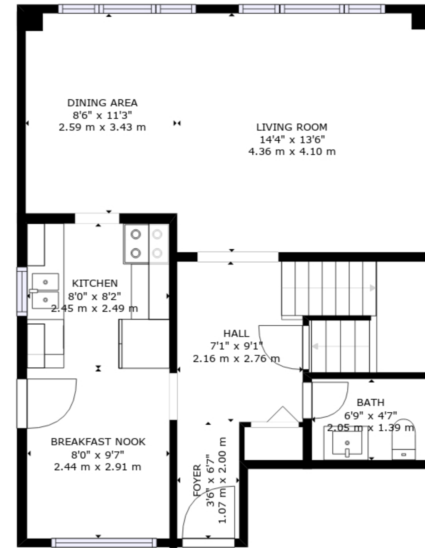
MAIN FLOOR
