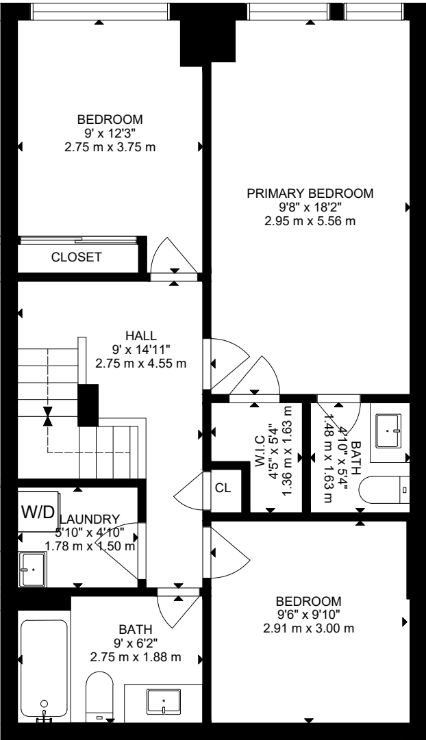
UPPER FLOOR
