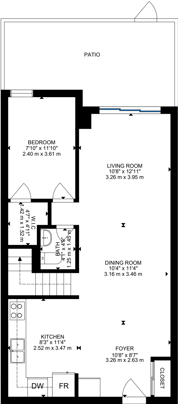
MAIN FLOOR
