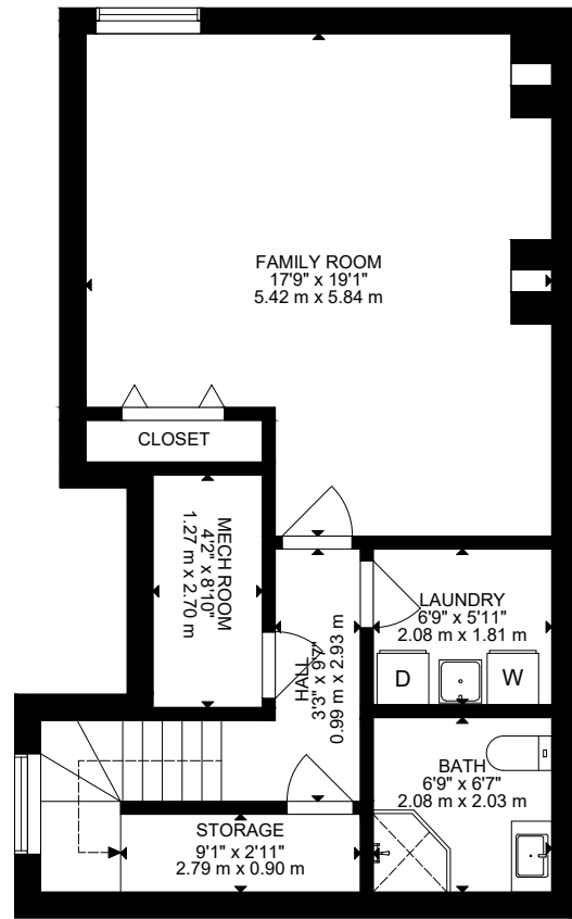
BASEMENT
