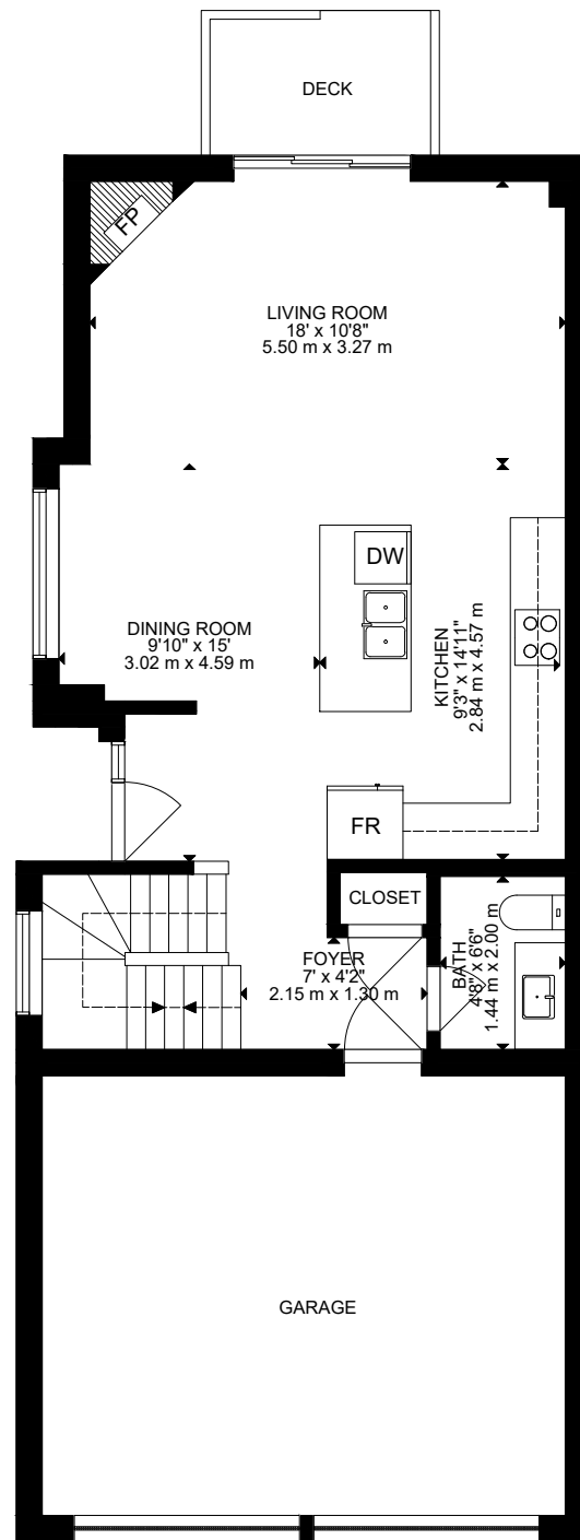
MAIN LEVEL
