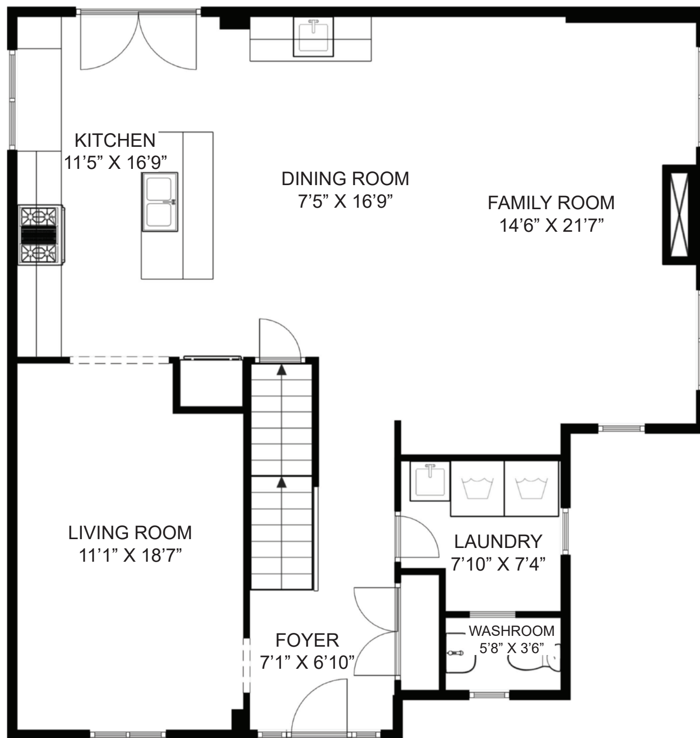
MAIN FLOOR
