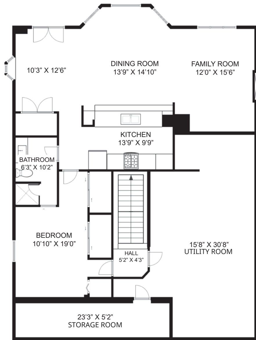
LOWER FLOOR
