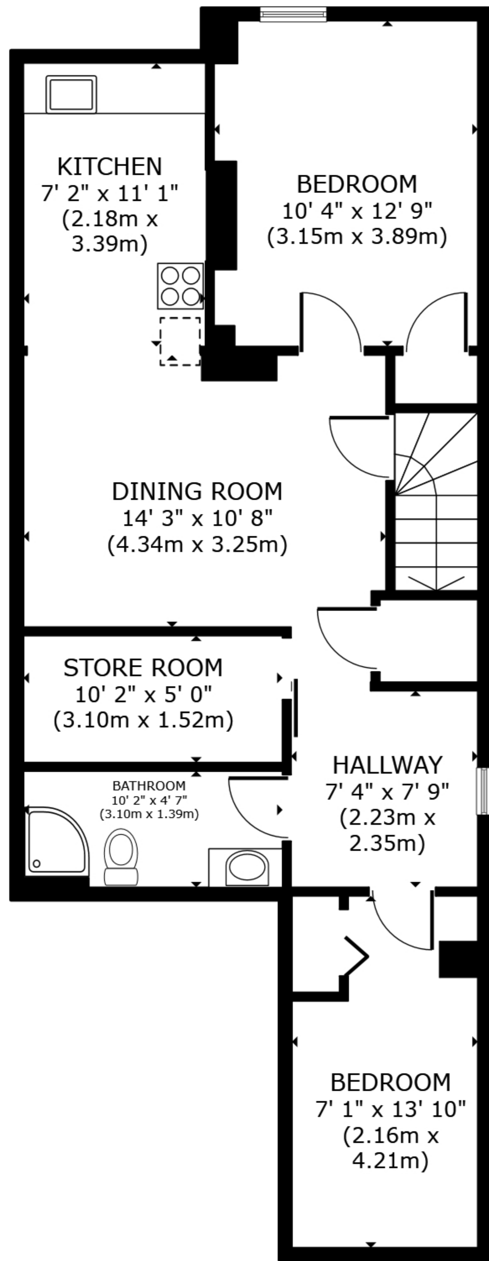
BASEMENT
