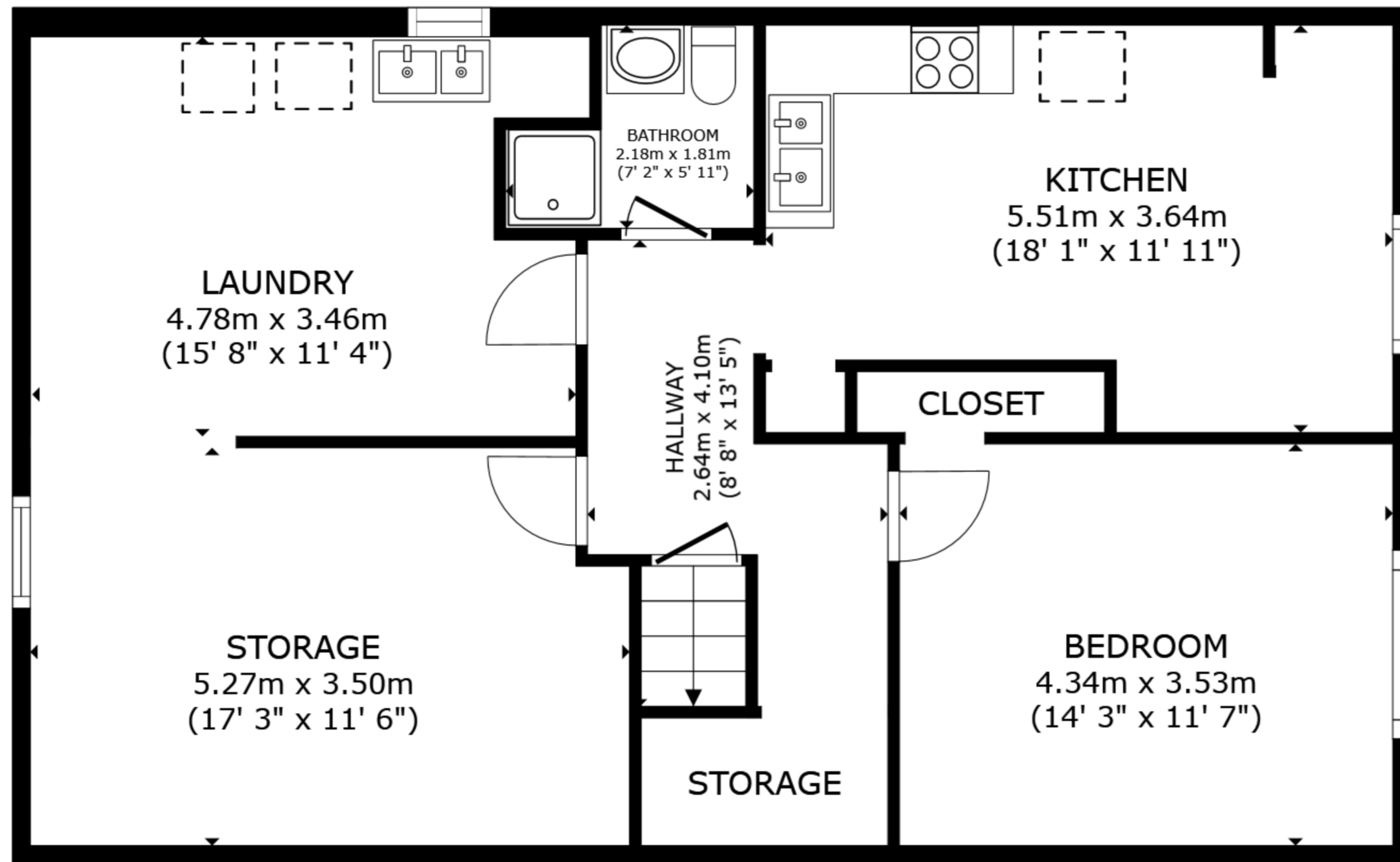
BASEMENT
