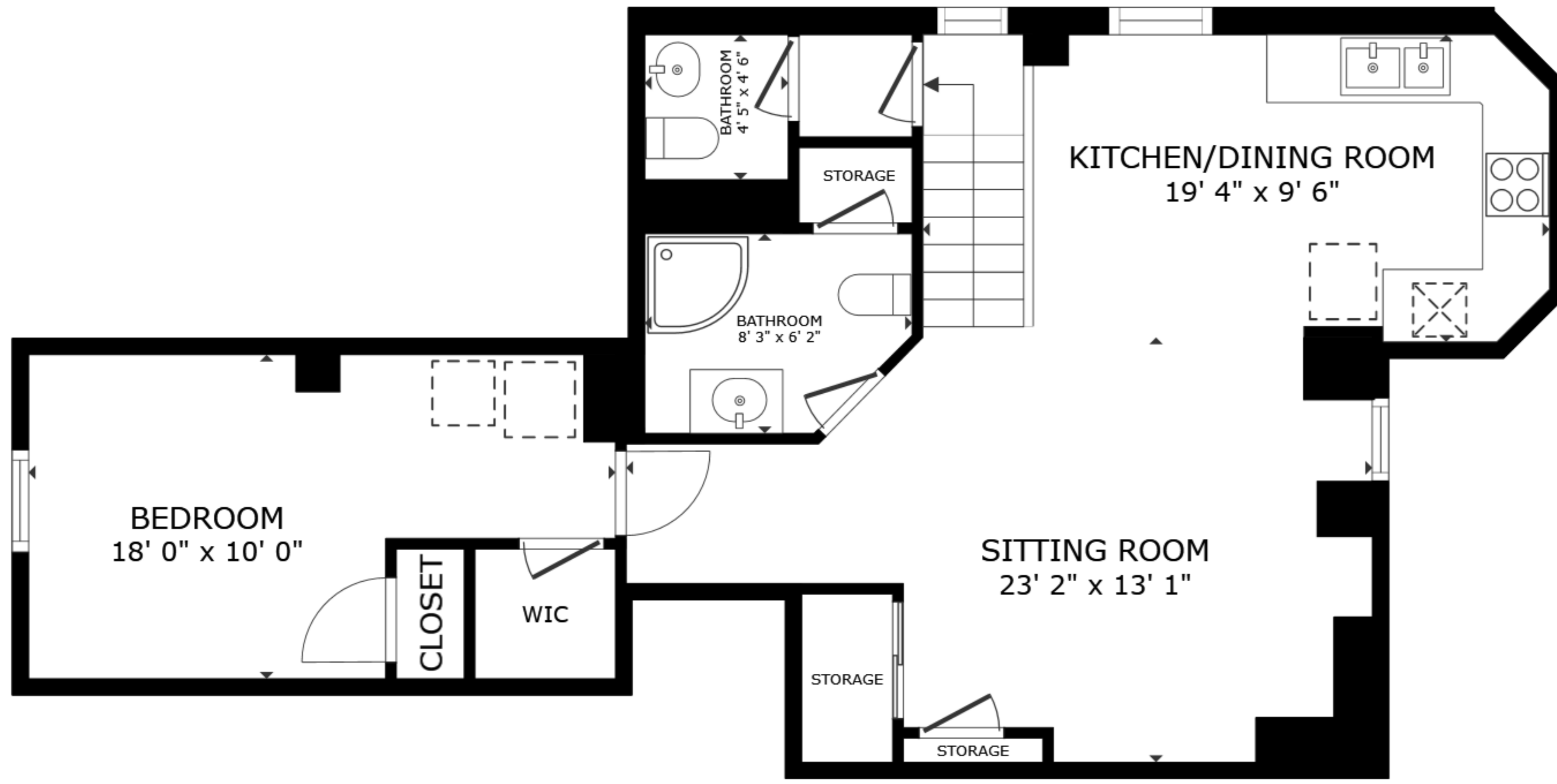
FLOOR 1
