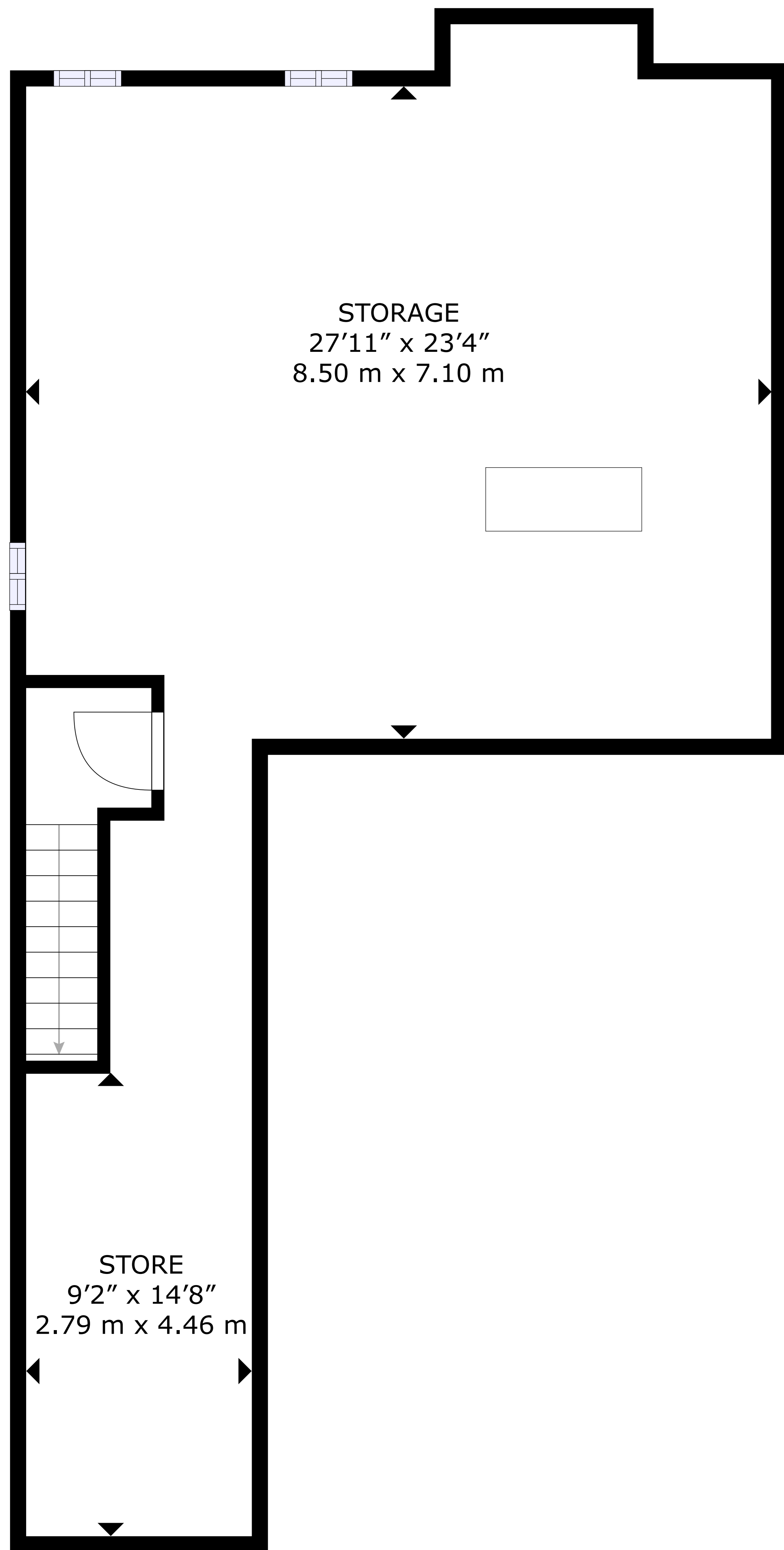
BASEMENT
