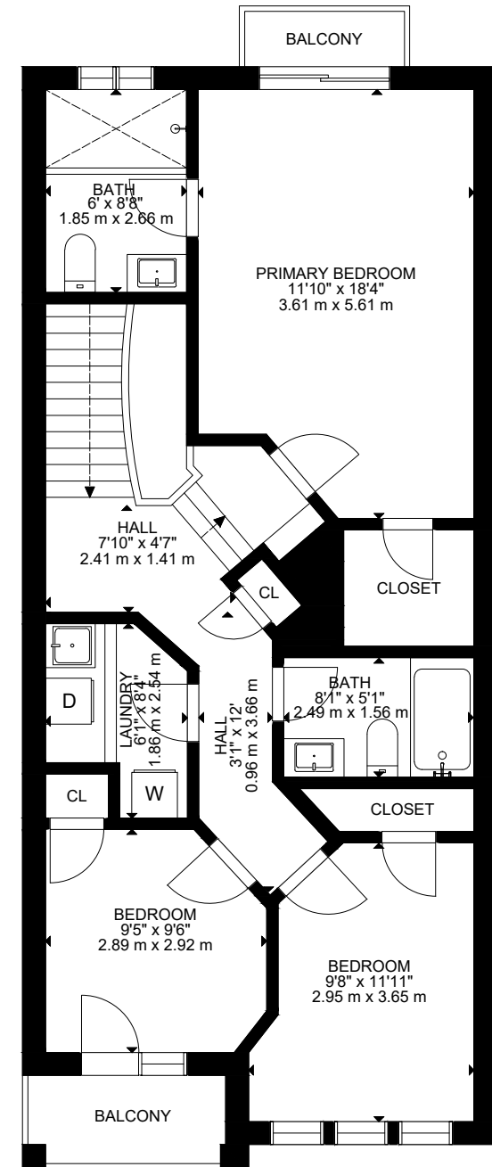
UPPER FLOOR
