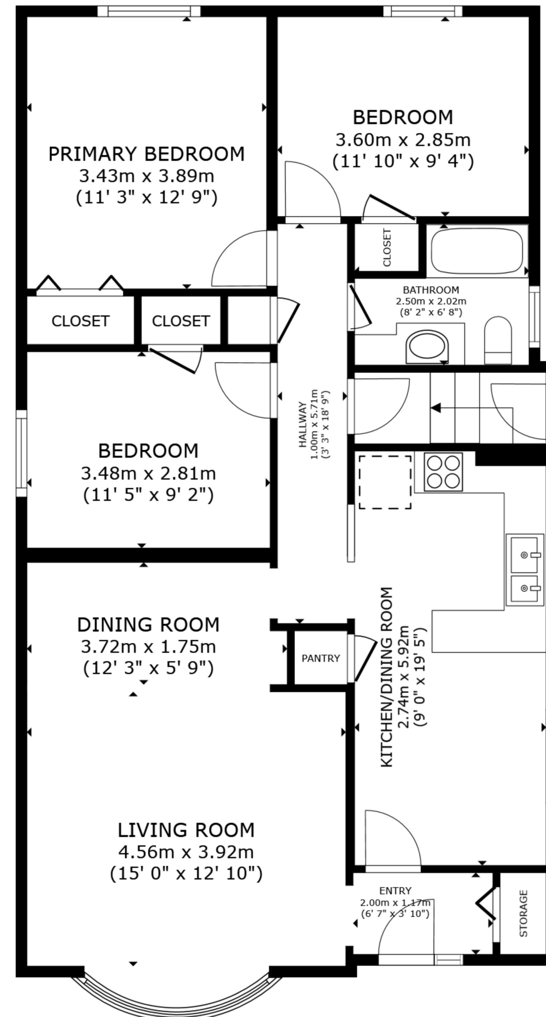
FLOOR 2
