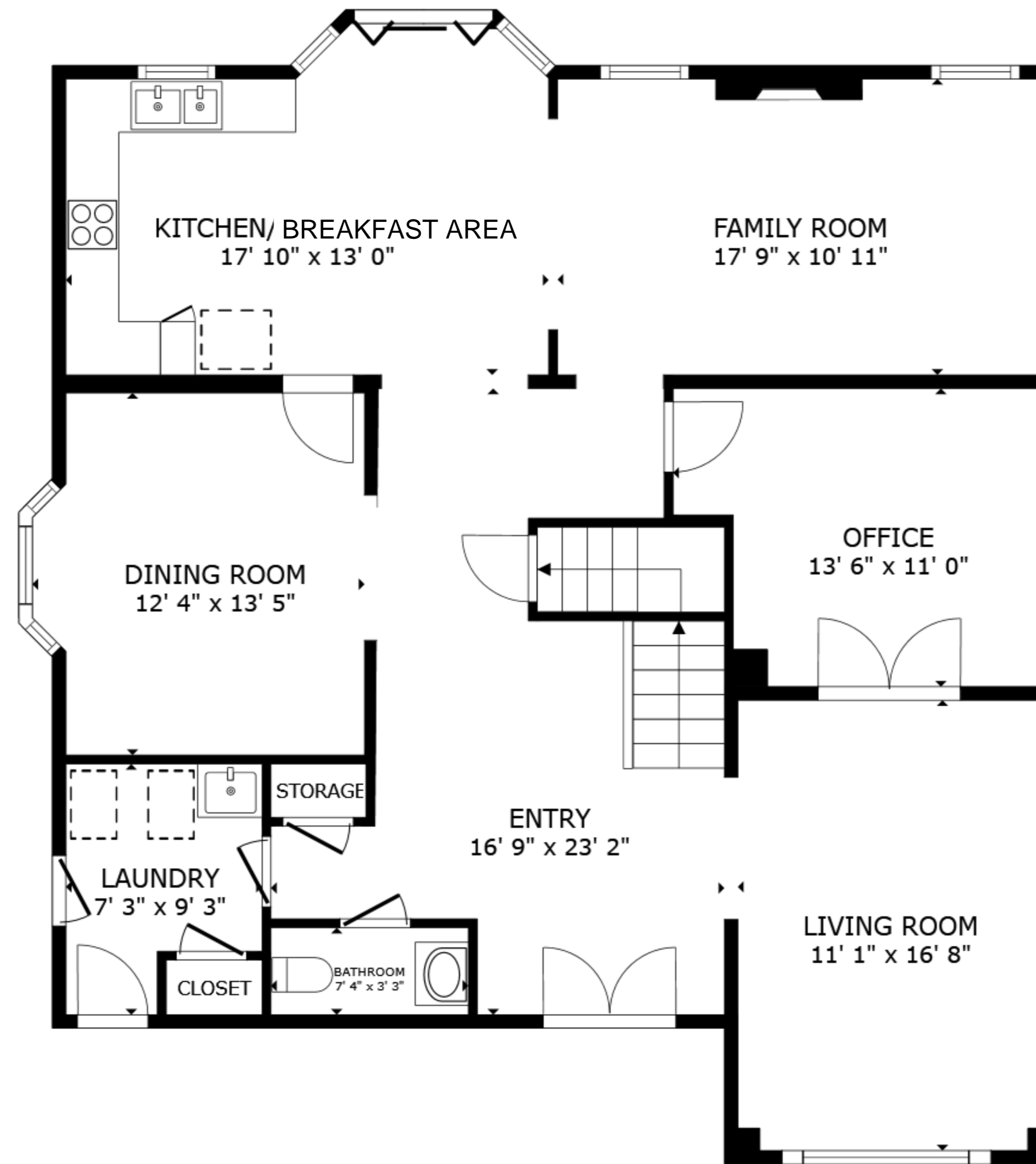
MAIN FLOOR
