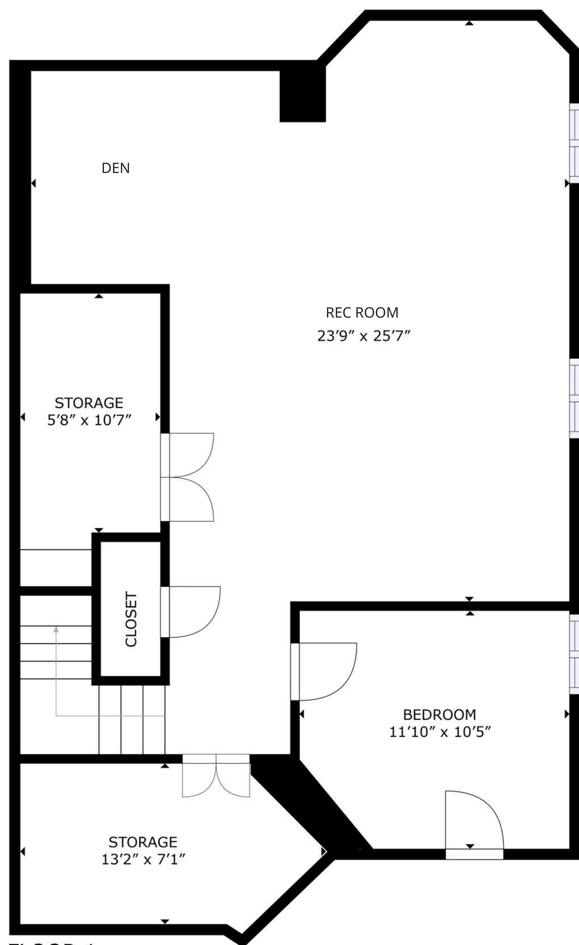
FLOOR 1
