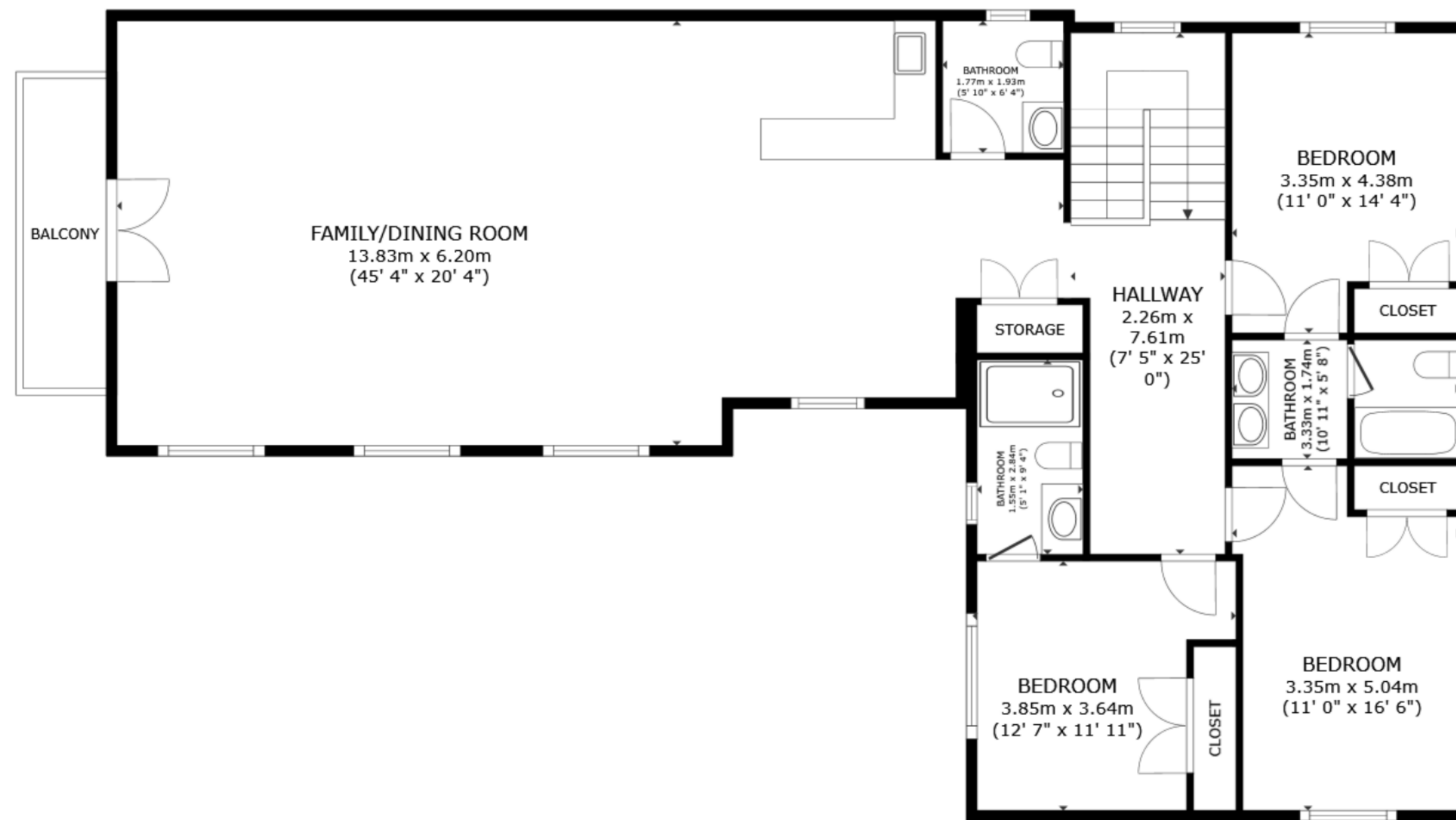
FLOOR 2
