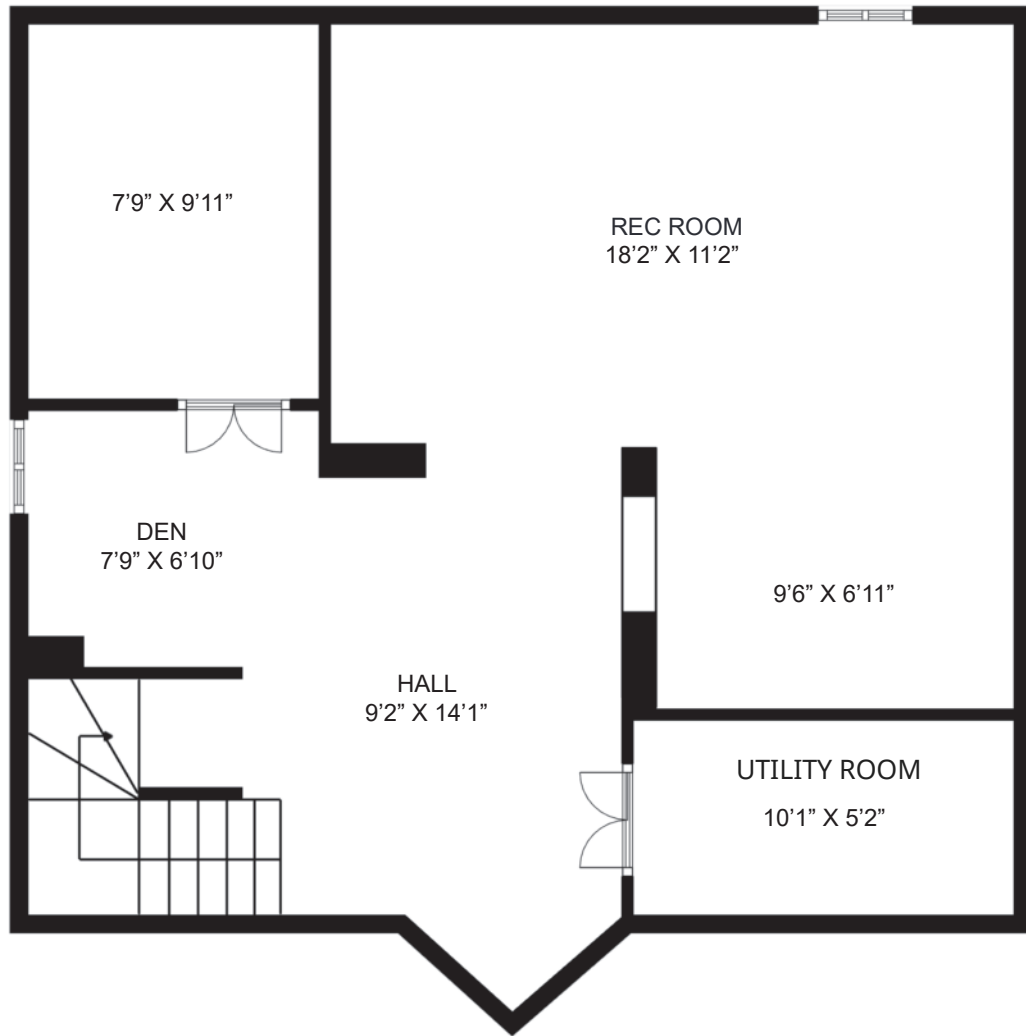
LOWER FLOOR
