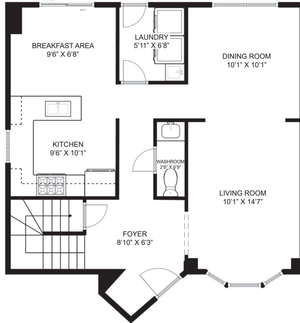
MAIN FLOOR
