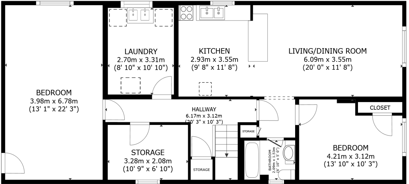
FLOOR 1
