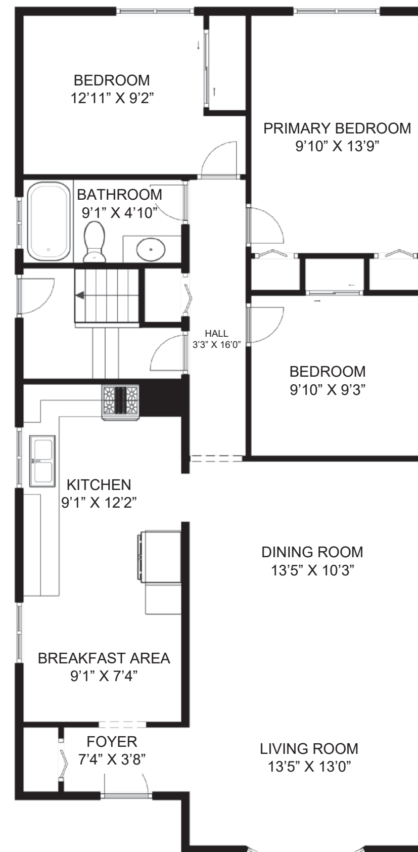
MAIN FLOOR
