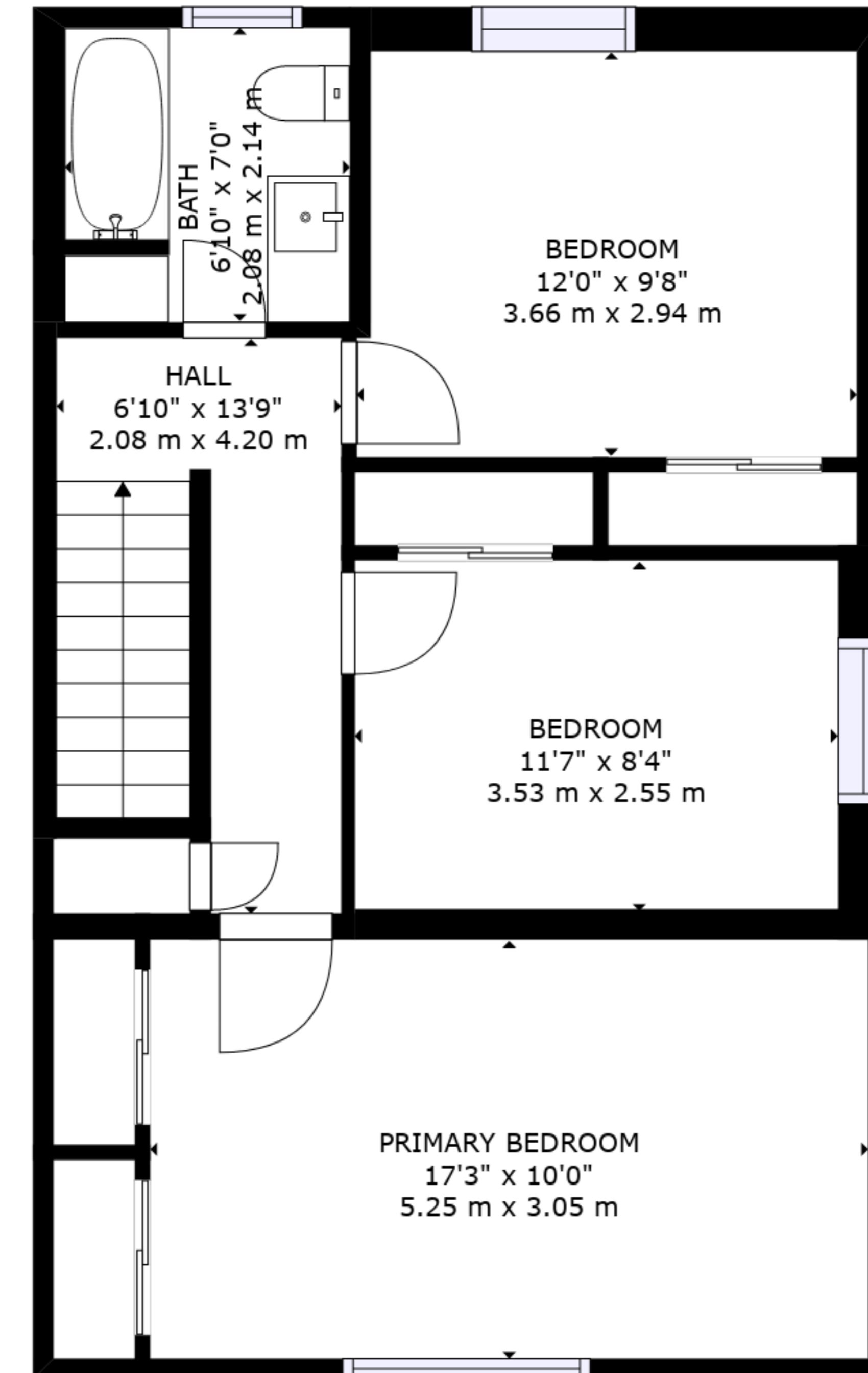
FLOOR 3
