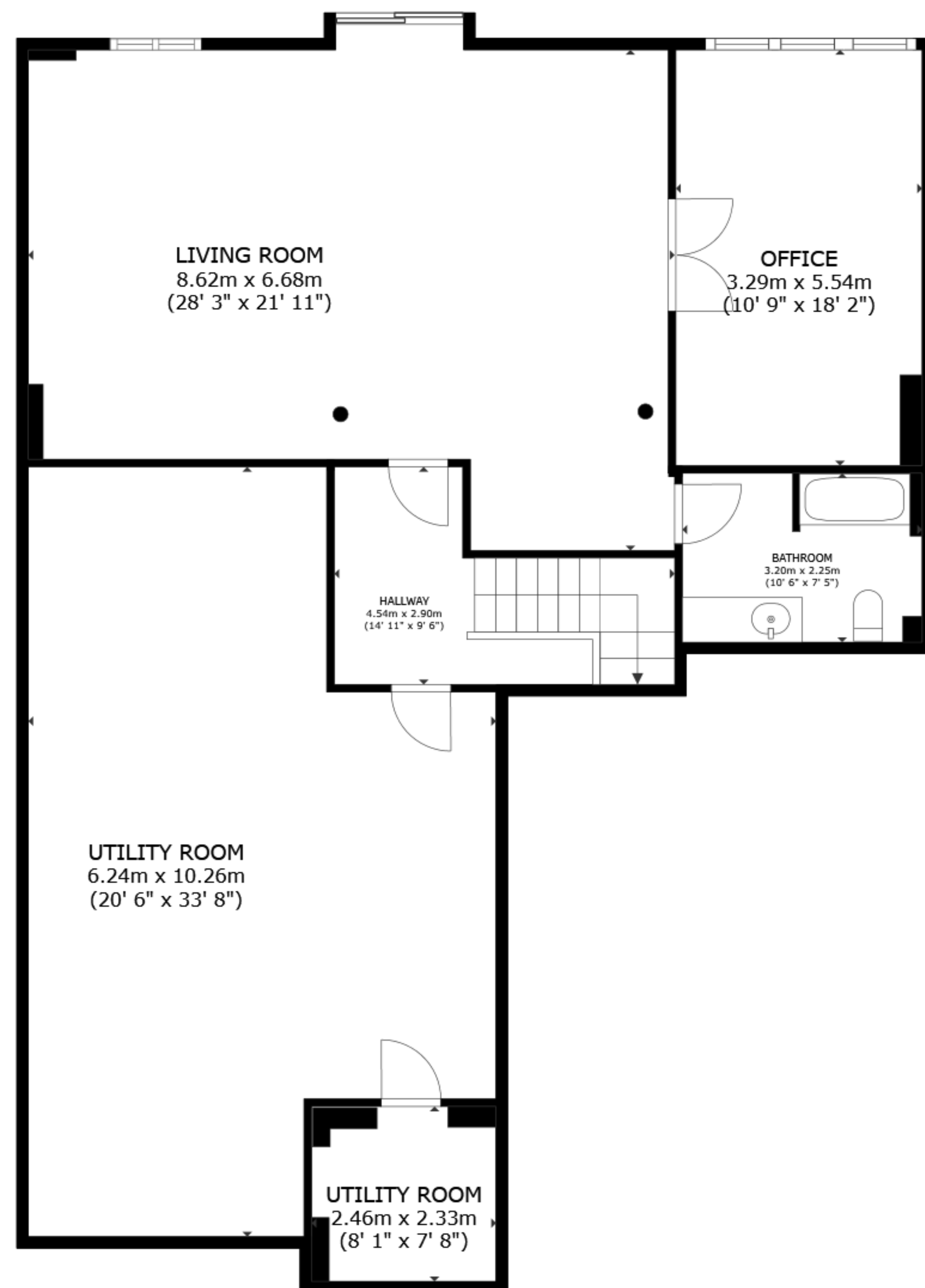
FLOOR 1
