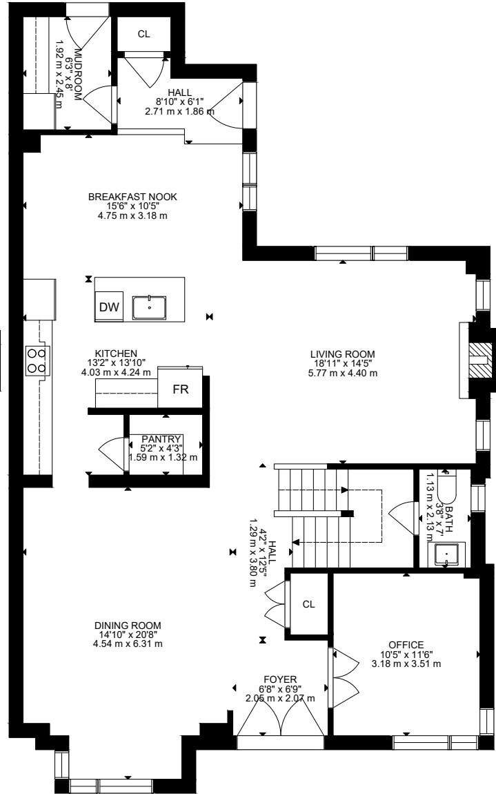
MAIN FLOOR
