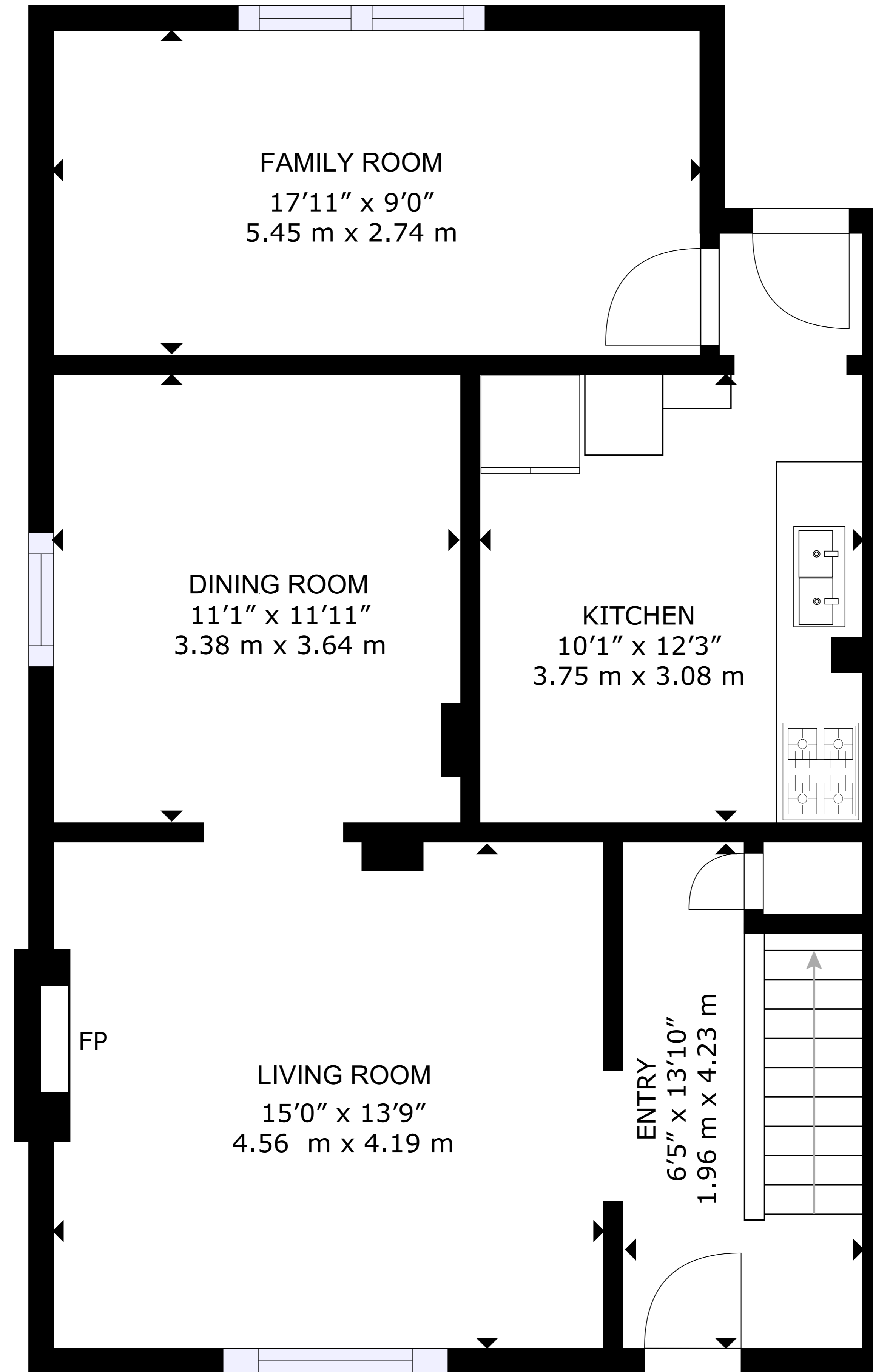
1ST FLOOR
