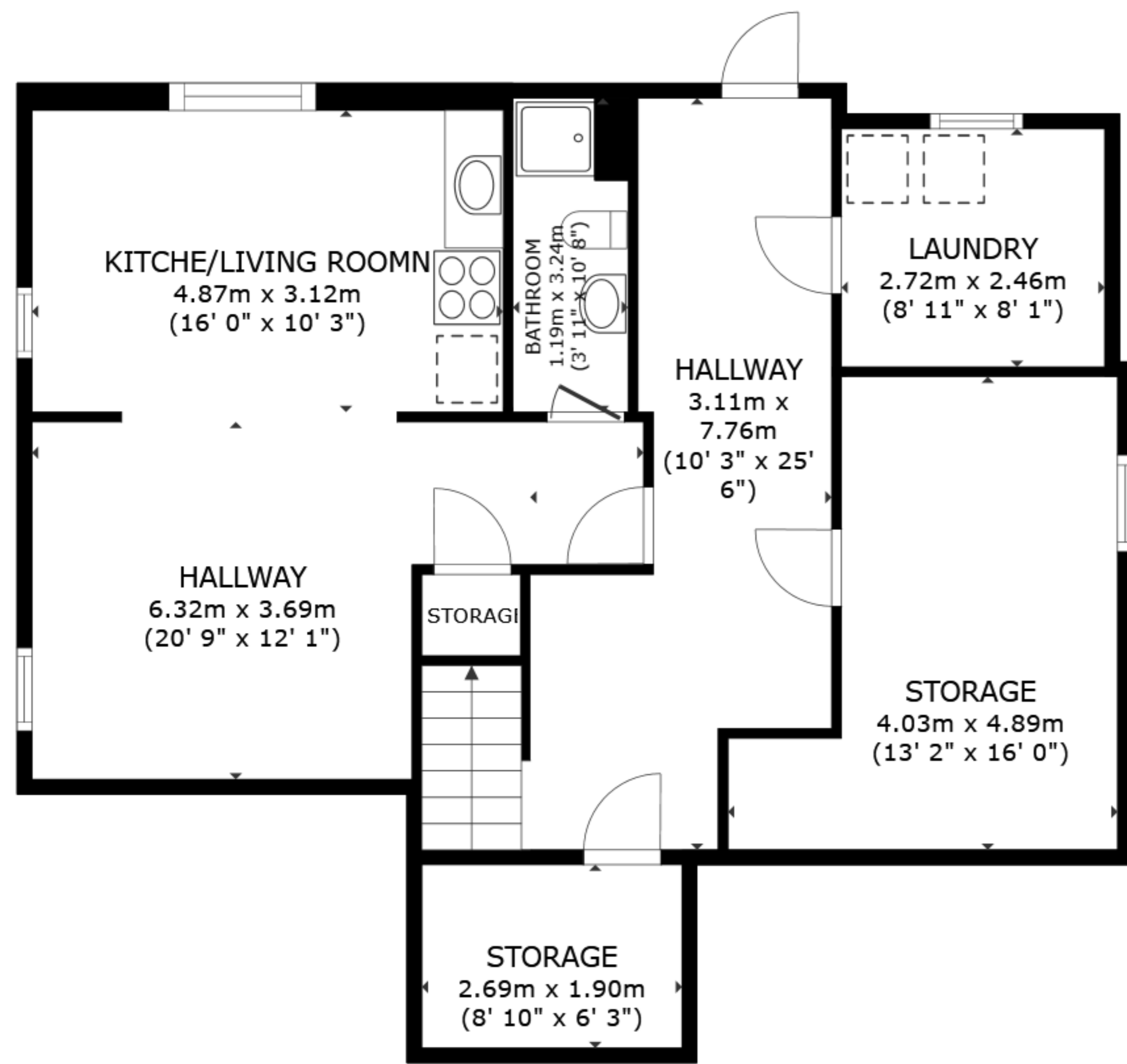
FLOOR 1
