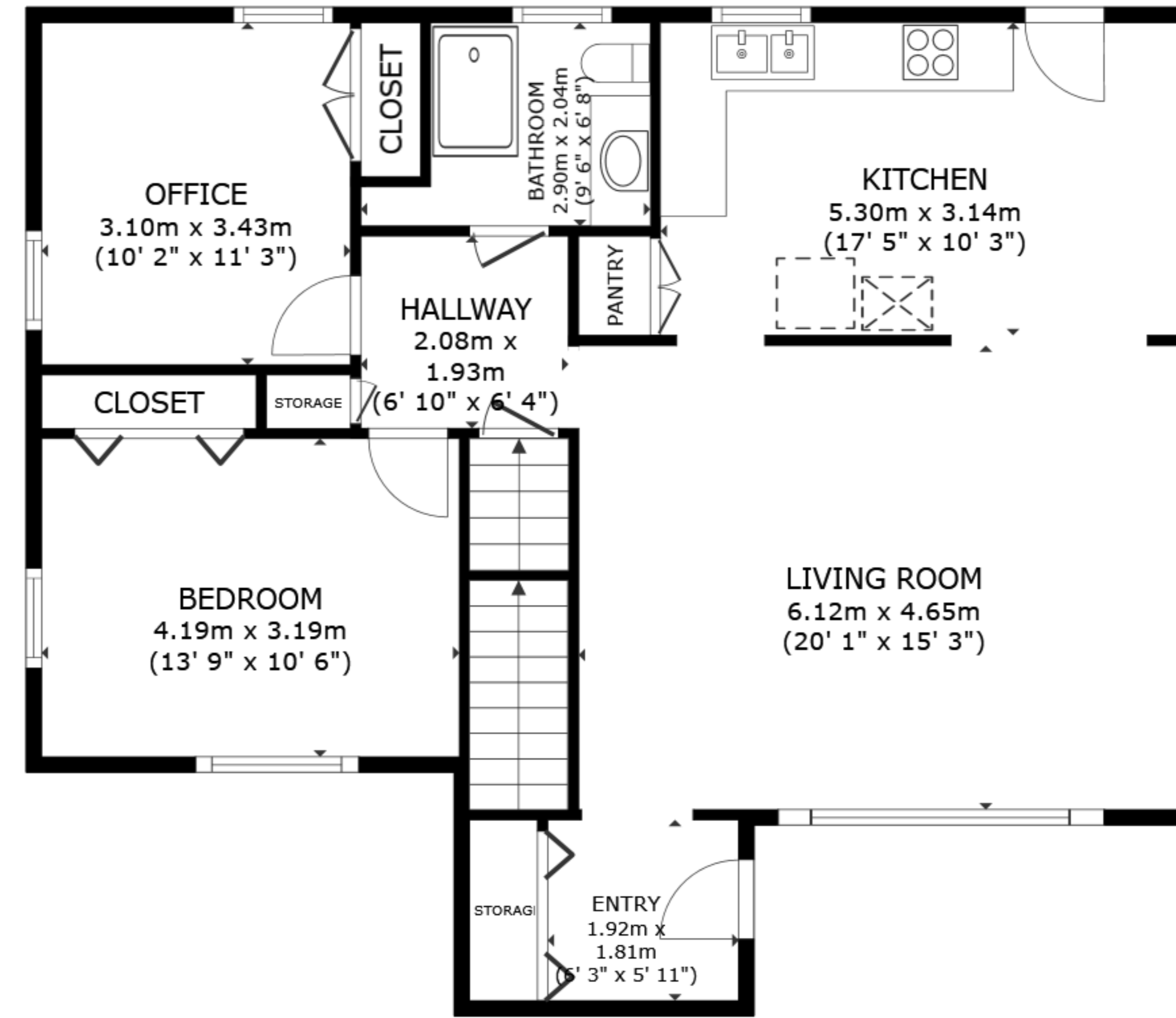
FLOOR 2
