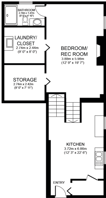
BASEMENT
