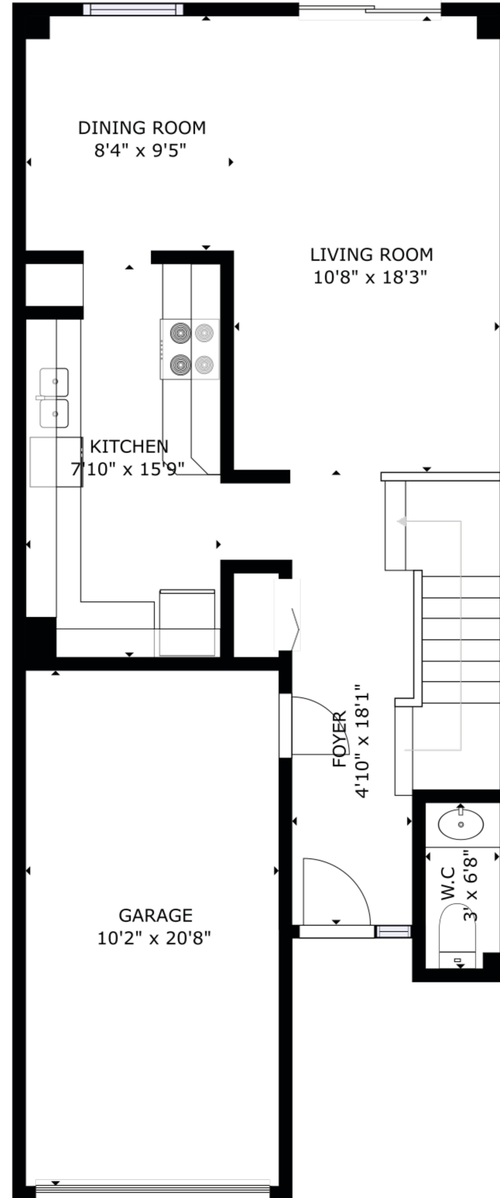
MAIN FLOOR
