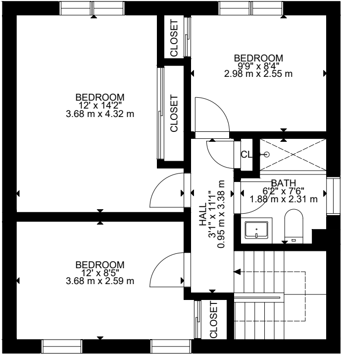
UPPER FLOOR
