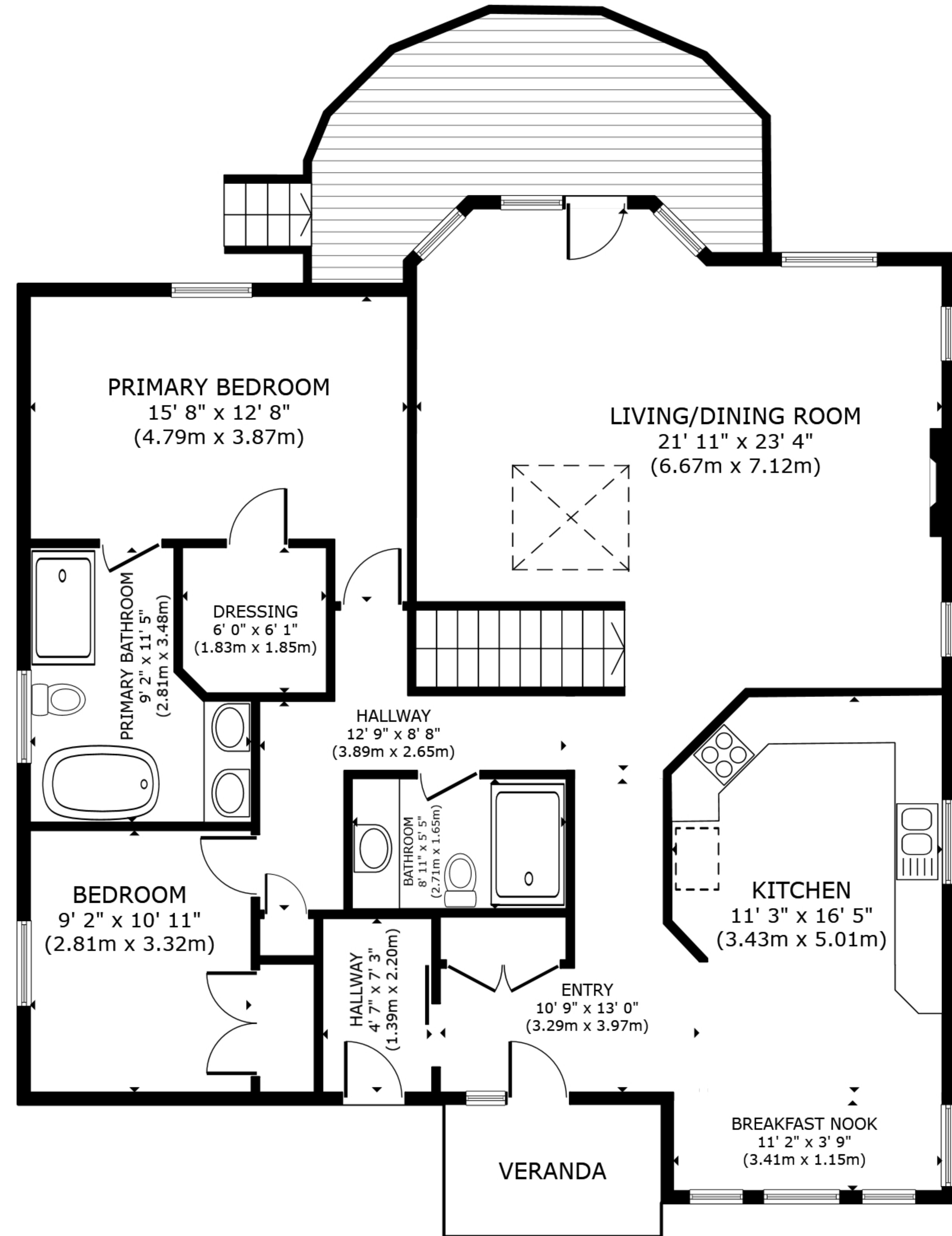
FLOOR 2
