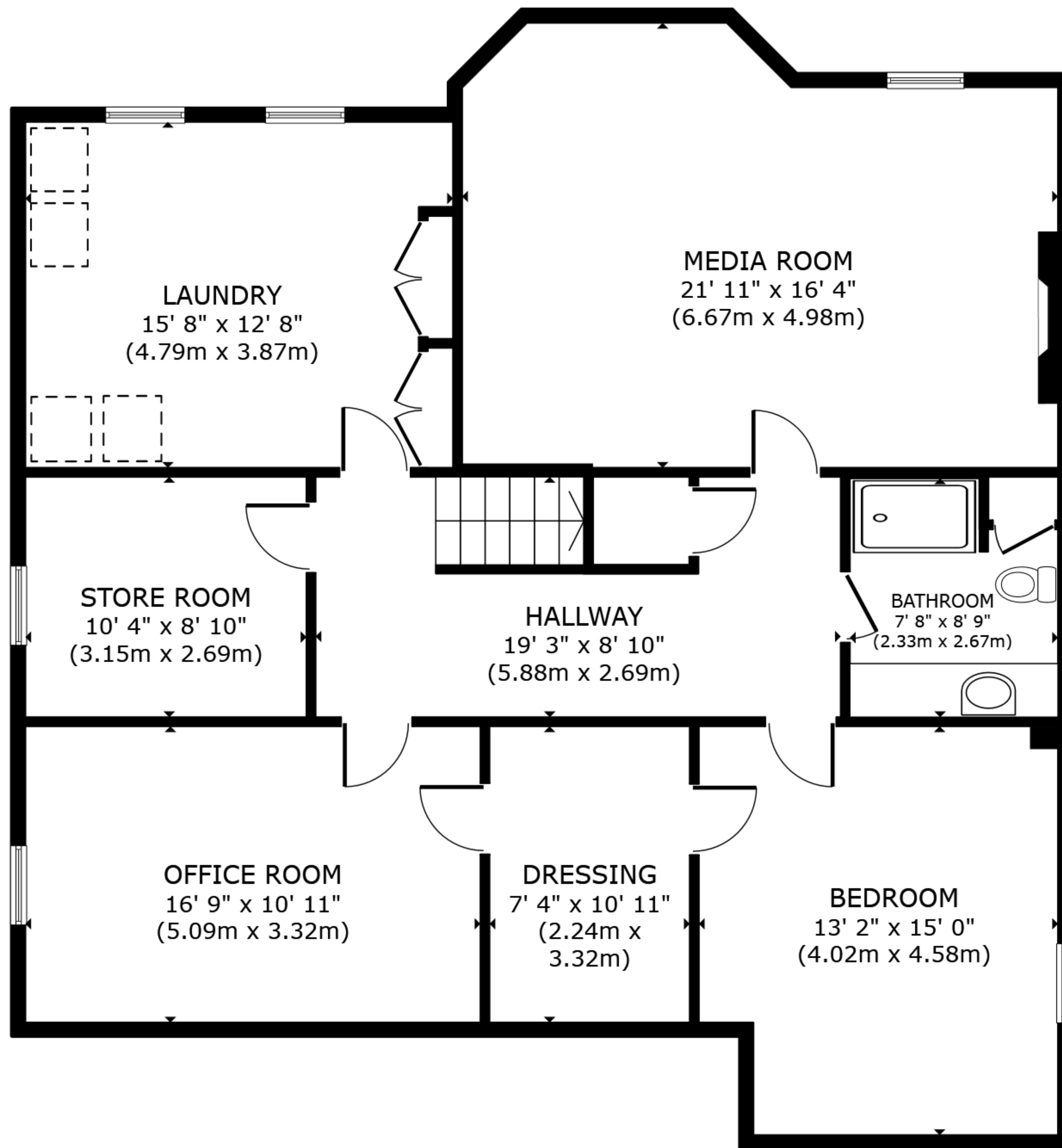
FLOOR 1
