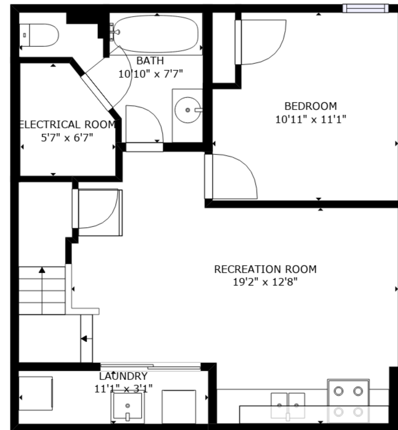
FLOOR 1
