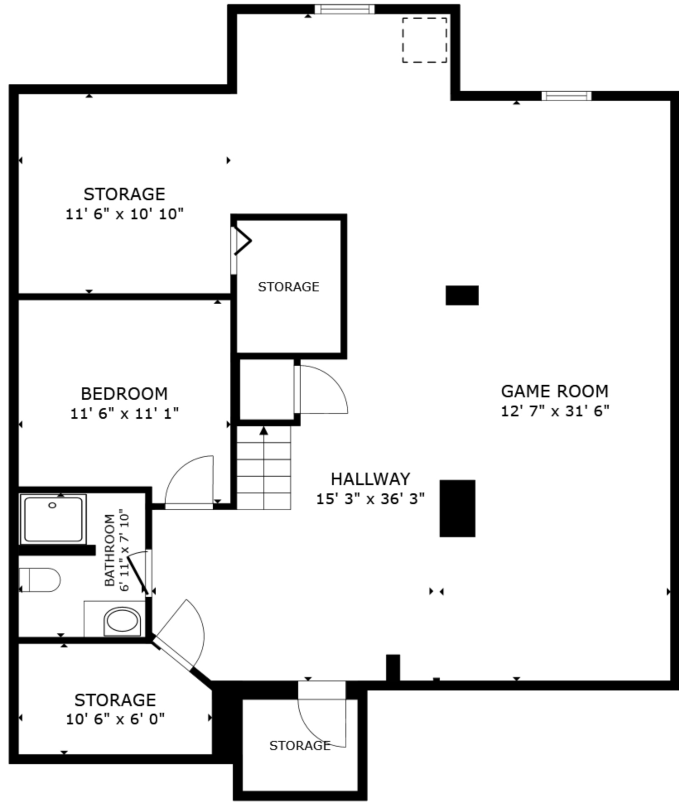
BASEMENT
