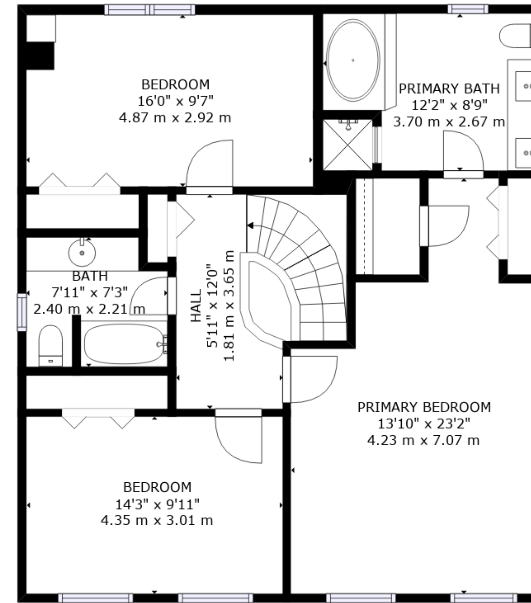
FLOOR 3
